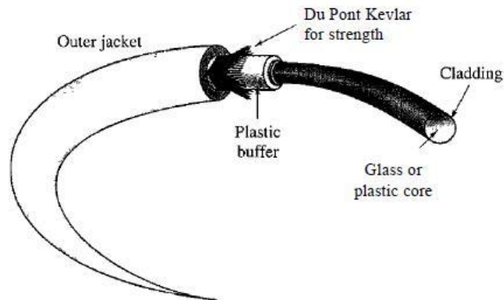
Figure 7.14 Fiber construction
