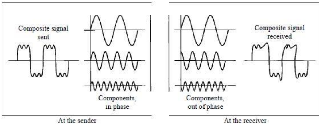
Figure 3.28 Distortion
