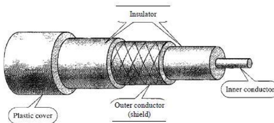
Figure 7.7 Coaxial cable
