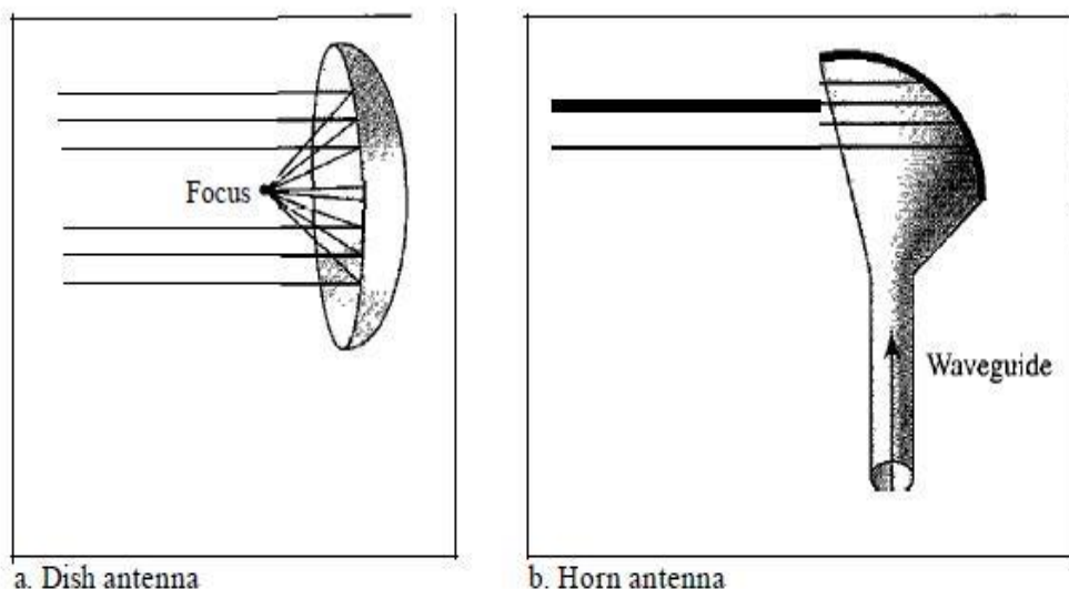
Figure 7.21 Unidirectional antennas
