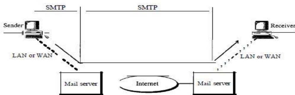
Figure 26.16 SMTP range
